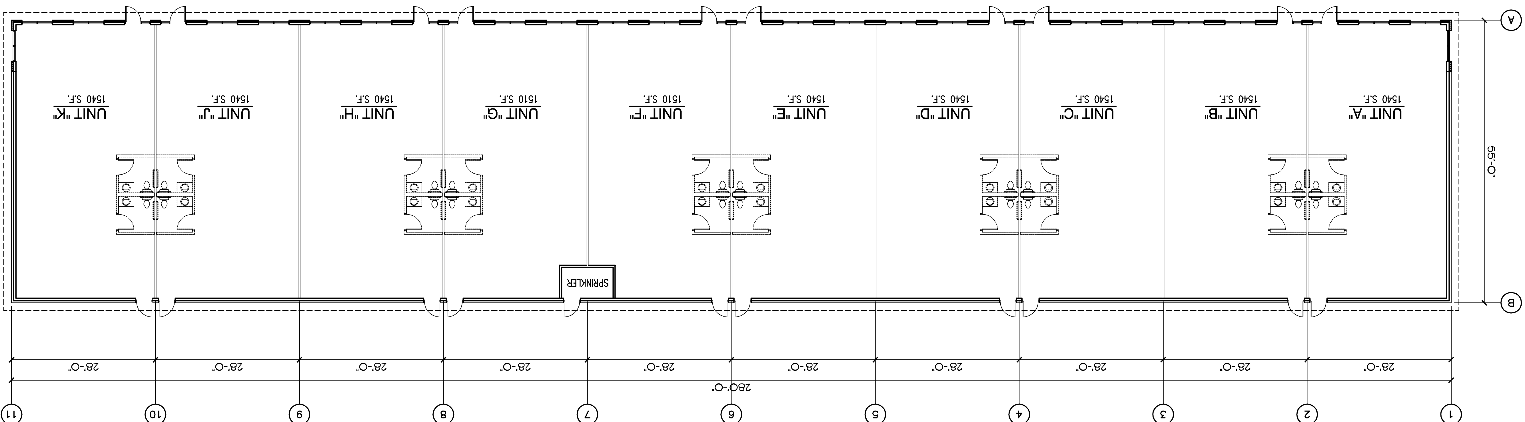
FLOOR PLAN SCALE 3/32" = 1'-0"
